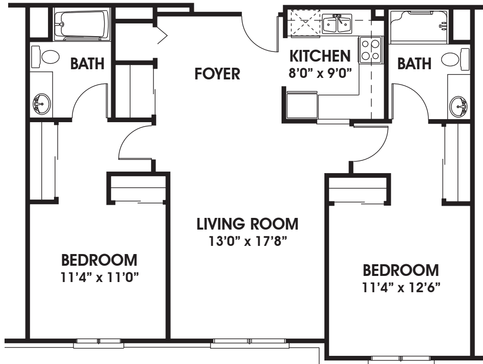
DOROTHY LOVE APARTMENTS TWO BEDROOM DELUXE UNIT 1023 S.F.
